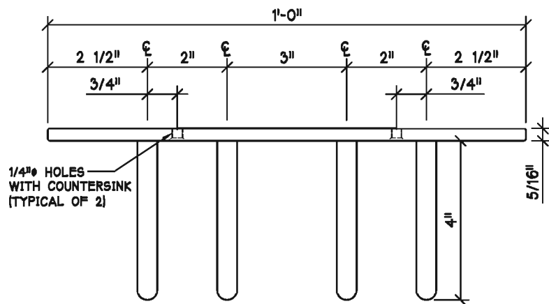
A 4-PEG APRON RACK PLAN VIEW
